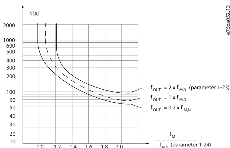
Illustration 31: ETR Characteristics
