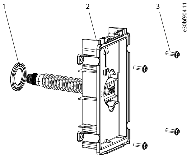
Illustration 49: Base Plate with Sub-D Connector
