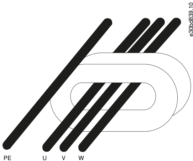
Illustration 18: Installing Common-mode Cores
