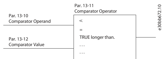
Illustration 35: Comparators
