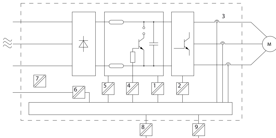
Illustration 80: Galvanic Isolation
